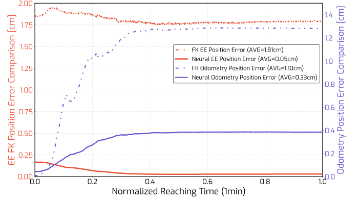
Fig. 7: Impact of neural forward models in the real world. We plot the neural and analytical forward kinematics and base odometry as a function of execution time steps. The plot shows 1 minute of execution at 50Hz.
